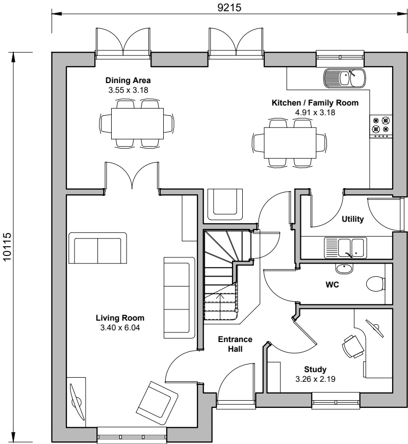
Ground Floor Floor Area 149.44m 2 - 1,609sqft
