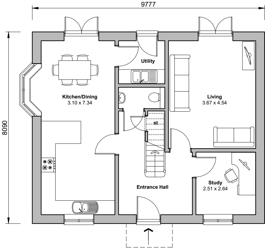
Ground Floor Floor Area 133.26m 2 - 1,434sqft
