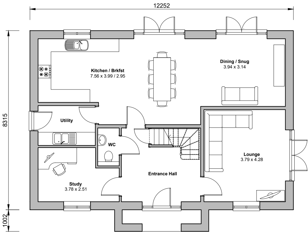
Ground Floor Floor Area 177.66m 2 - 1,912sft
