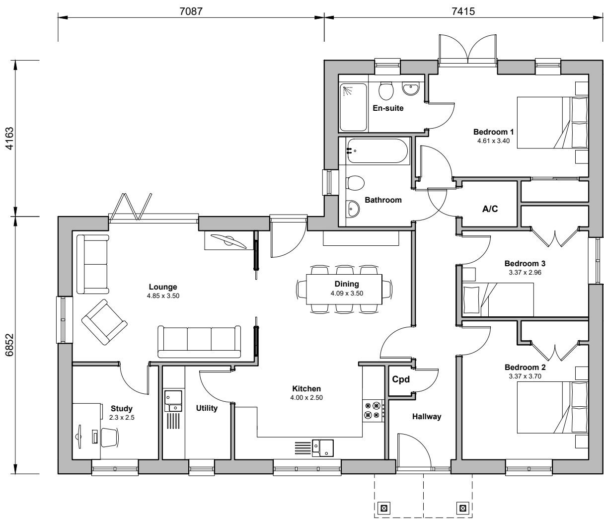
Ground Floor Floor Area 111.66m 2 - 1,202sft
